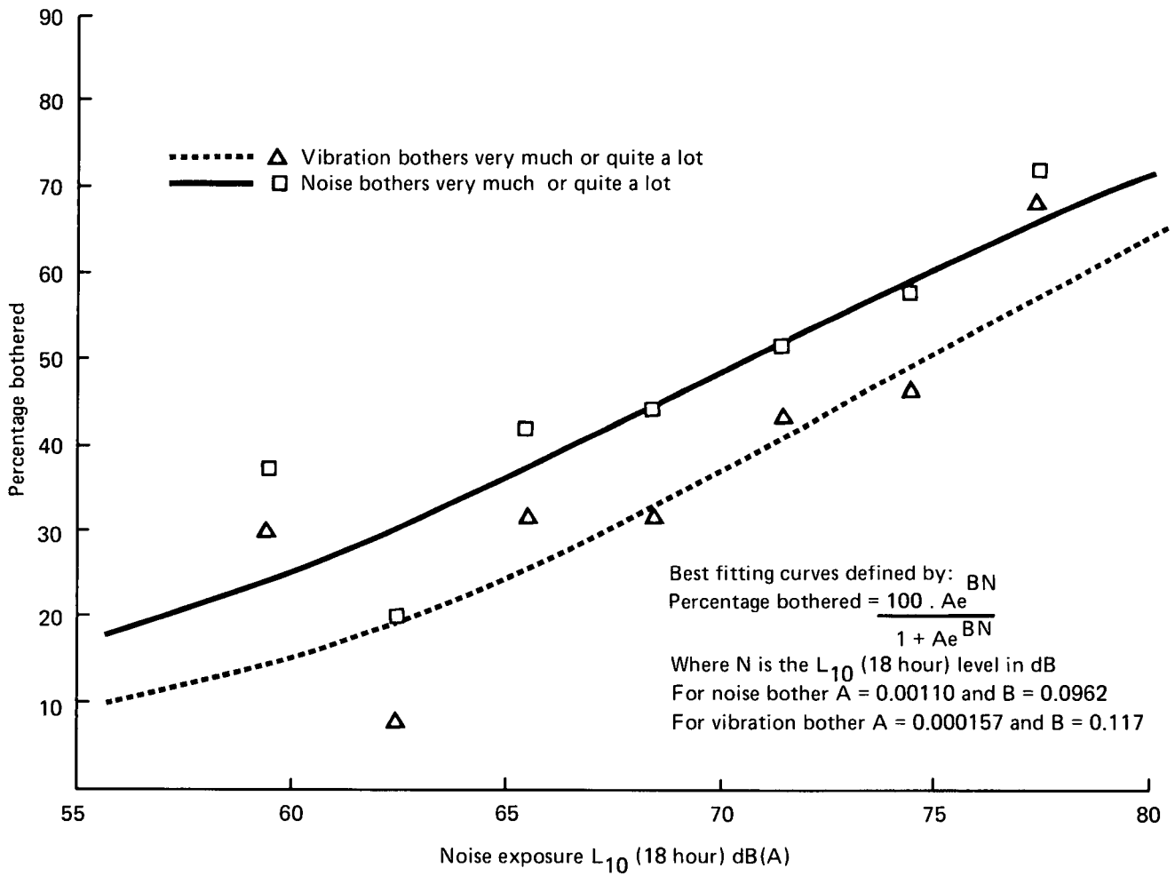
Fig.3 Percentages of respondents bothered by noise and vibration caused by traffic
