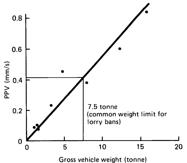
Fig.7 Variation of vertical peak particle velocity at 6m with gross vehicle weight for loaded 2 axle vehicles crossing a 0.6 x 25mm hump at 48 km/h
