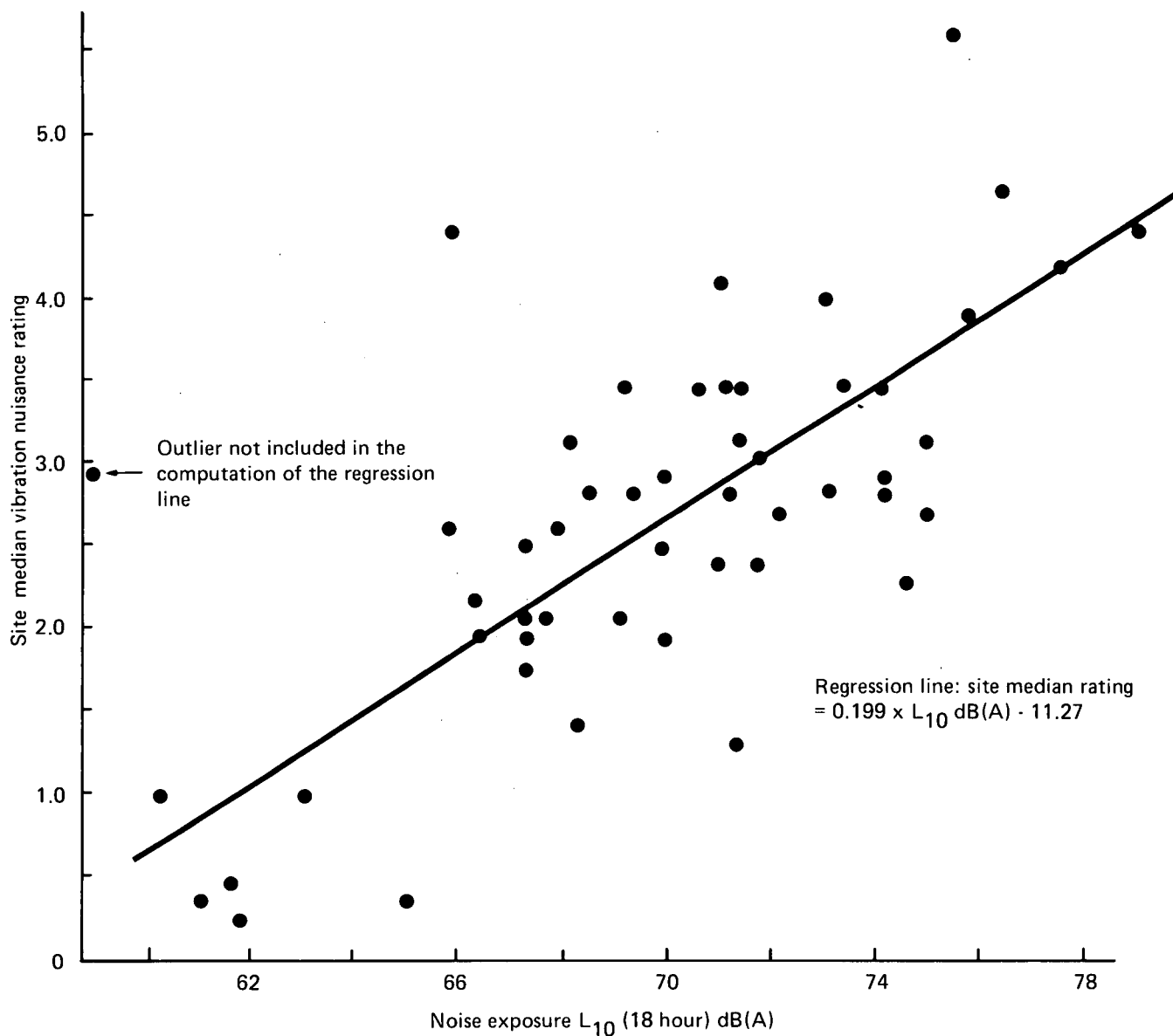
Fig.4 Median vibration nuisance rating and L 10 (18 hour) dB(A)
