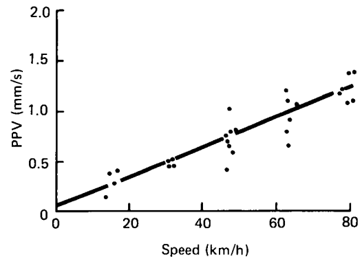
Fig.6 Vertical PPV at 6m with vehicle speed over 0.6m x 25mm hump - TRRL hump
