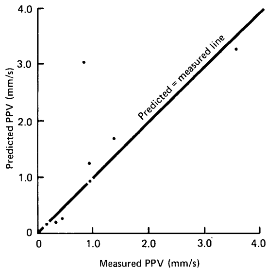
Fig.10 Measured and predicted maximum vertical PPVs at building foundations due to HGVs passing over road surface irregularities
