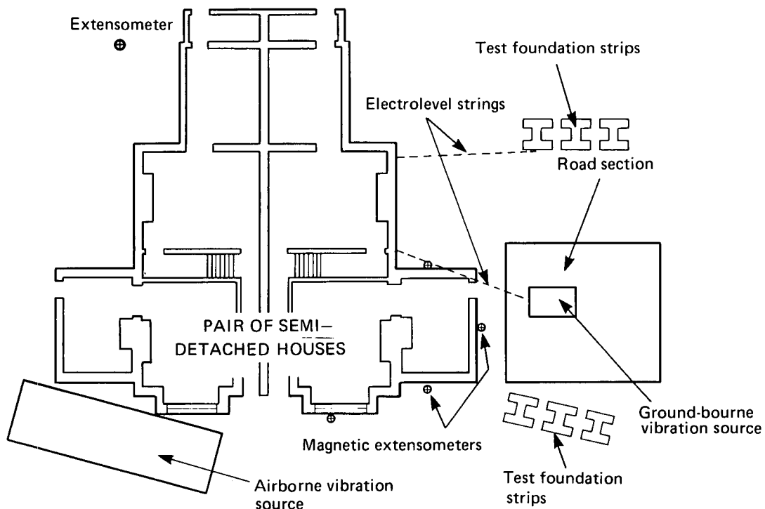
Fig.11 Site layout for fatigue test of a pair of semi-detached houses
