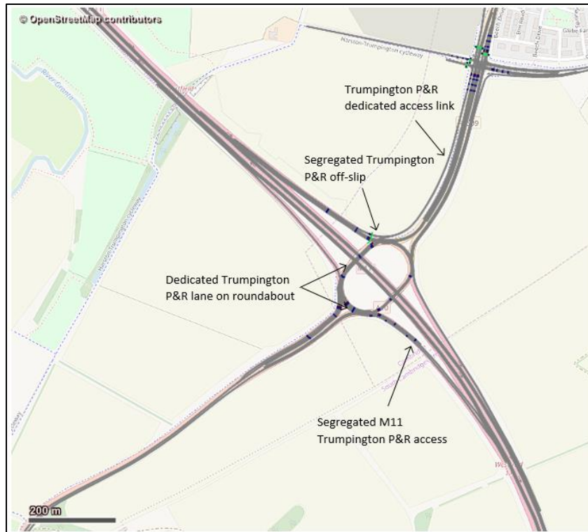
Figure 5.2 - Magenta M11 Junction 11 layout
