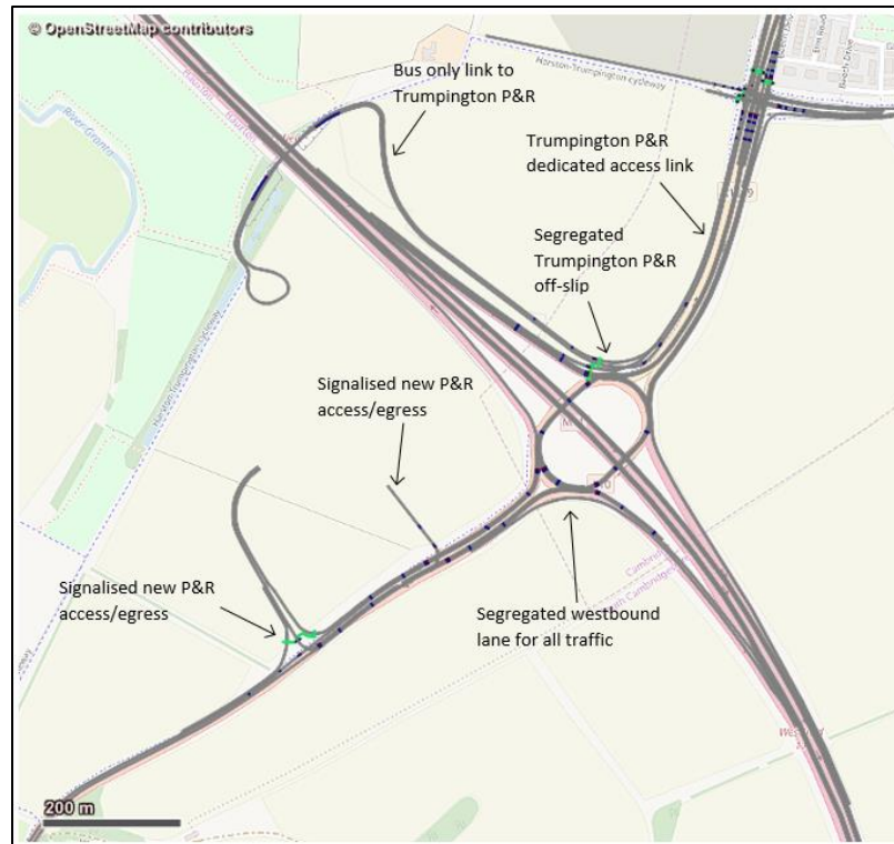
Figure 5.5 - Yellow M11 Junction 11 layout
