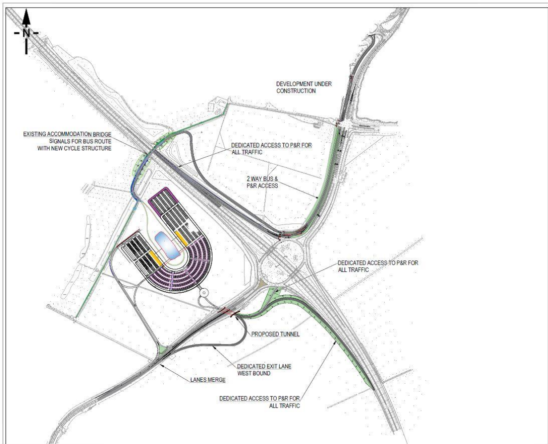
Figure 7: Cyan Scheme drawing
