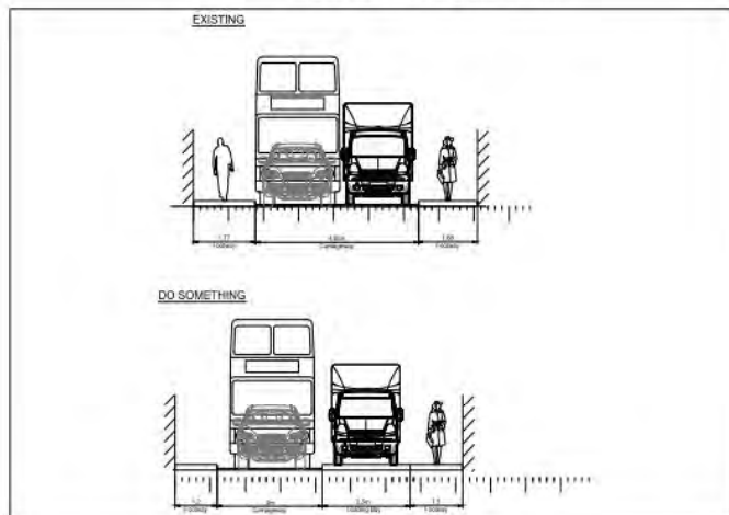
LOADING BAY-TYPICAL CROSS SECTION
